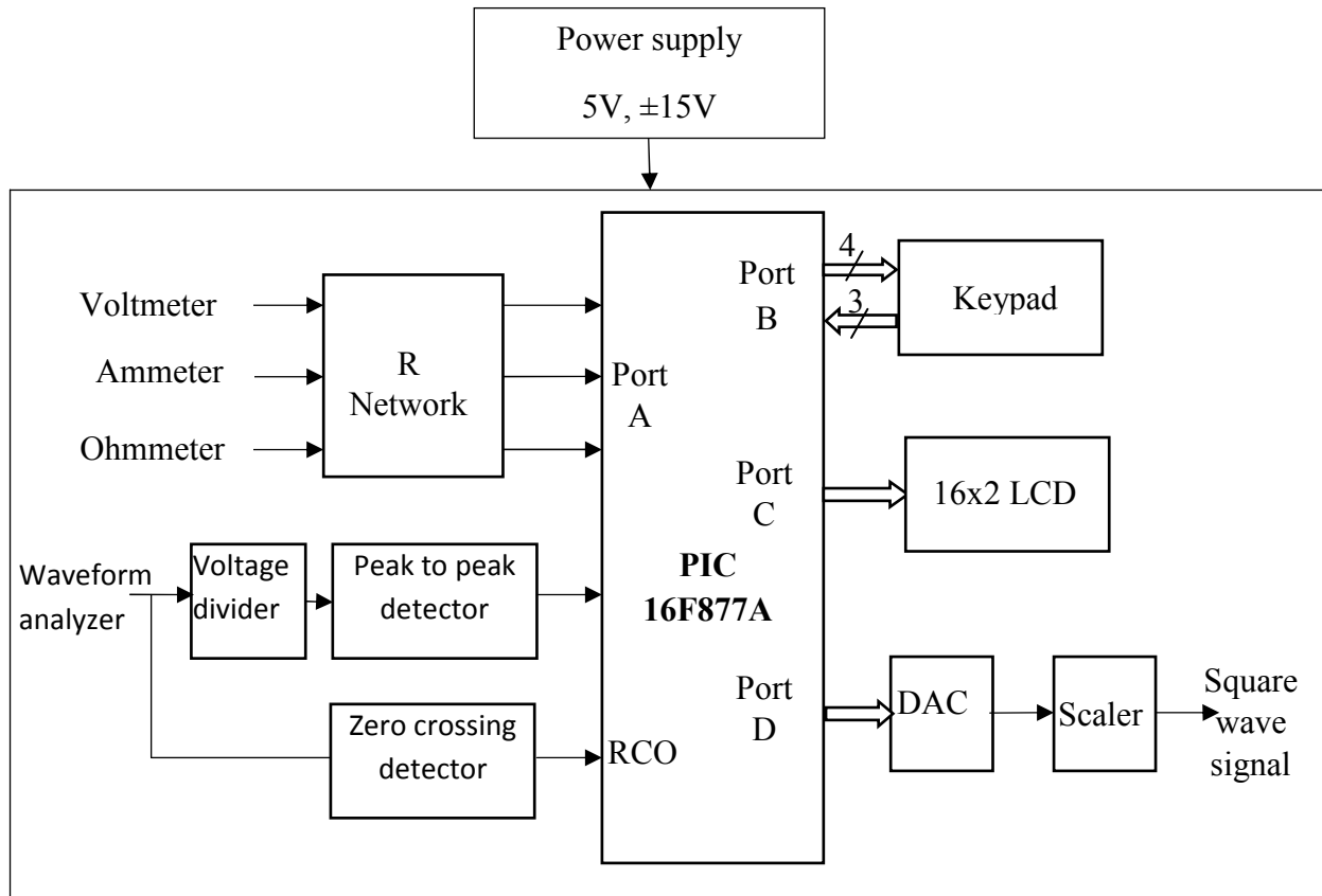
Figure 1 Block Diagram
