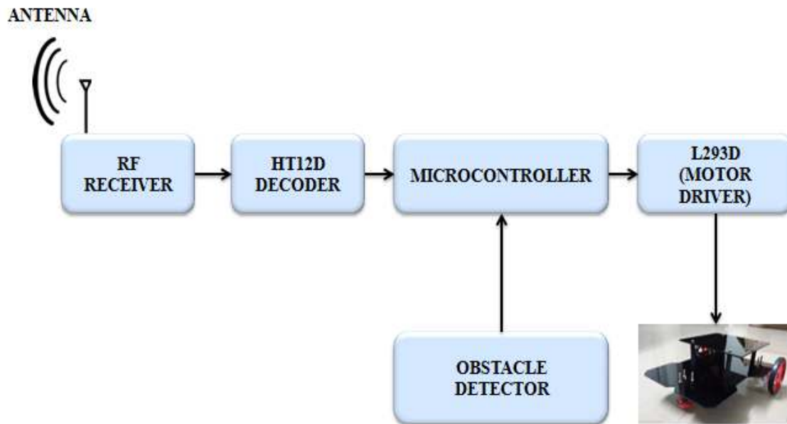
Block diagram of Receiver section
