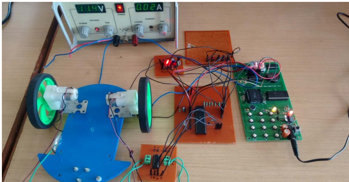
Figure 2: Prototype of the wheelchair
