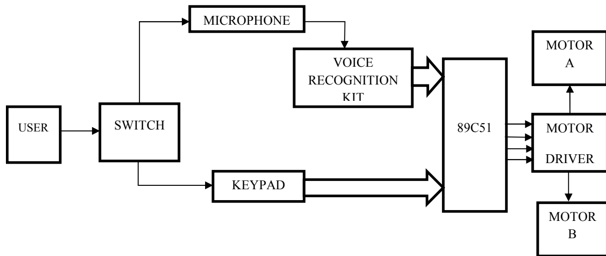
Figure 1: Block Diagram
