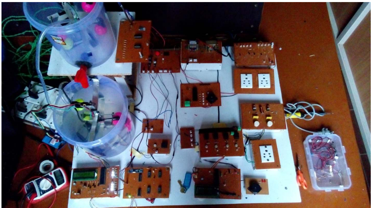
Figure 2: Experimental setup of the laboratory prototype
