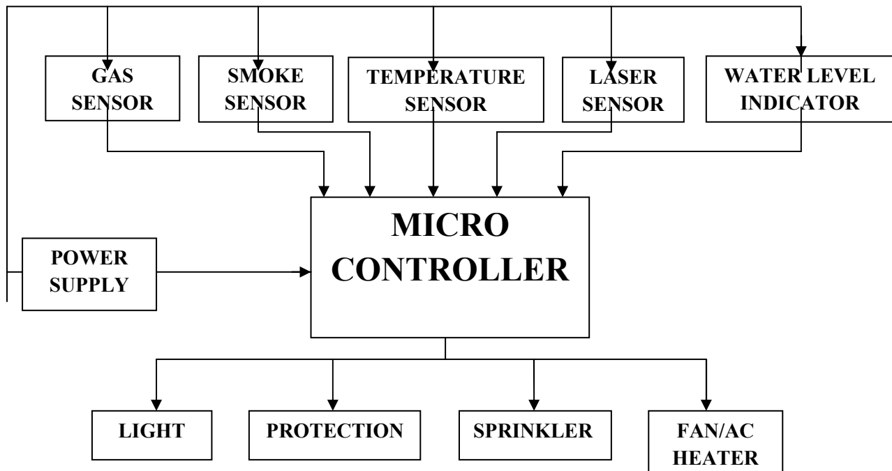
Figure 1: Block Diagram of ISWEEP smart house
