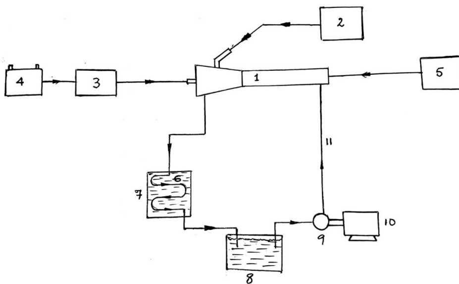
Schematic Representation of Cooling System of a Pulse Jet Engine
